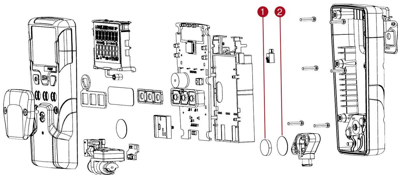
Figure 16. Replacing a Sensor or Sensor Filter for the SST4 Pump
